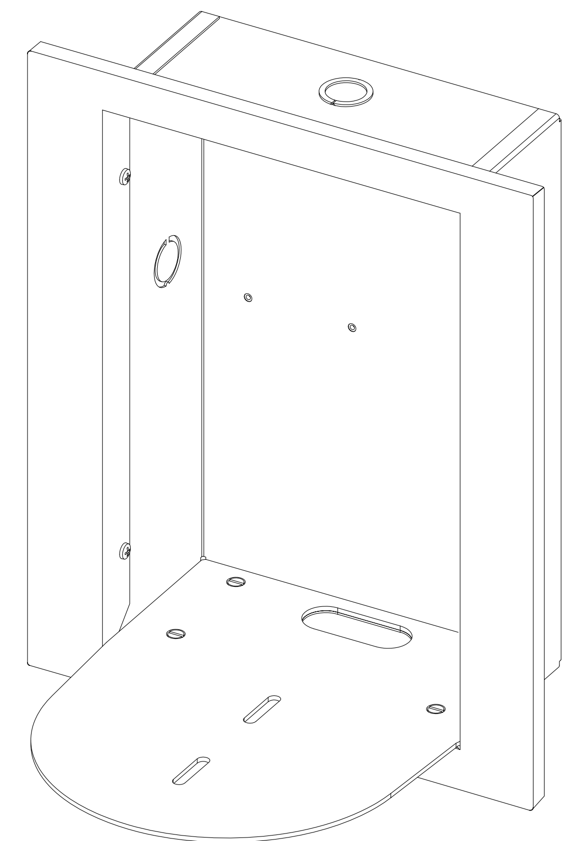
CAMERA BOX, PLATFORM AND FRAME ISO VIEW (NO SCALE)
