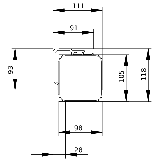
Case Side Detail
