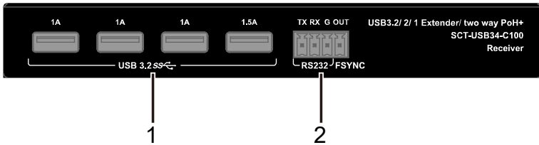
Front Panel
