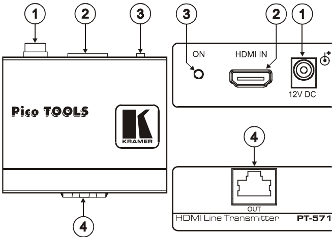
Figure 1: PT-571 HDMI Line Transmitter
