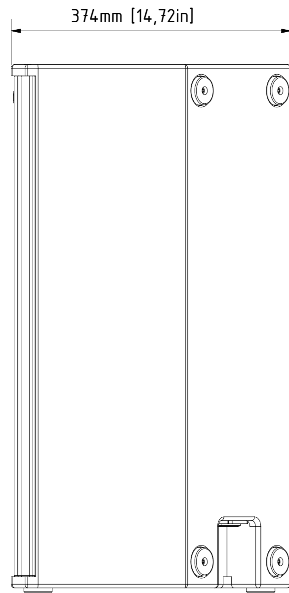
right view
