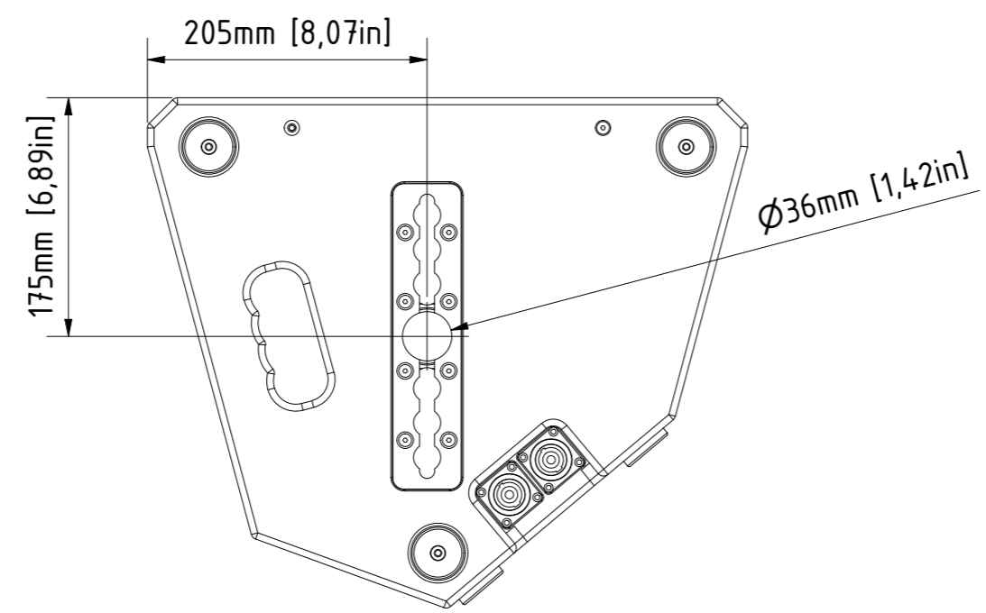
bottom view
