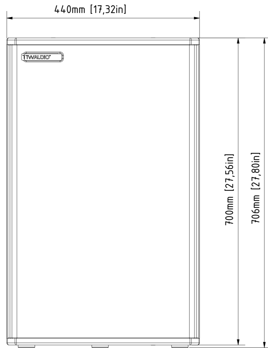
front view
