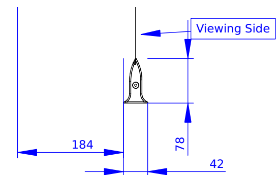
Case Side Detail
