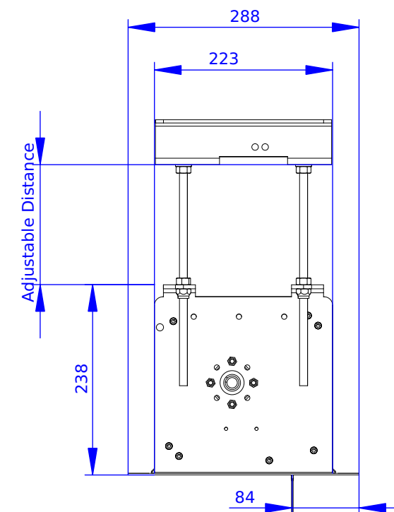
Case Side Detail
