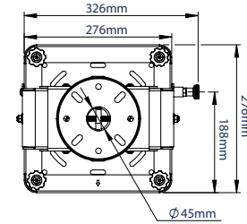
TOP VIEW WITH CEILING PLATE
