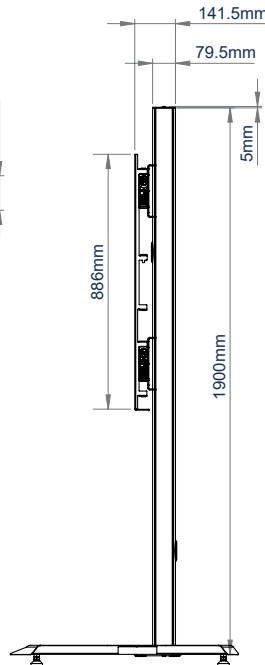
SIDE VIEW
