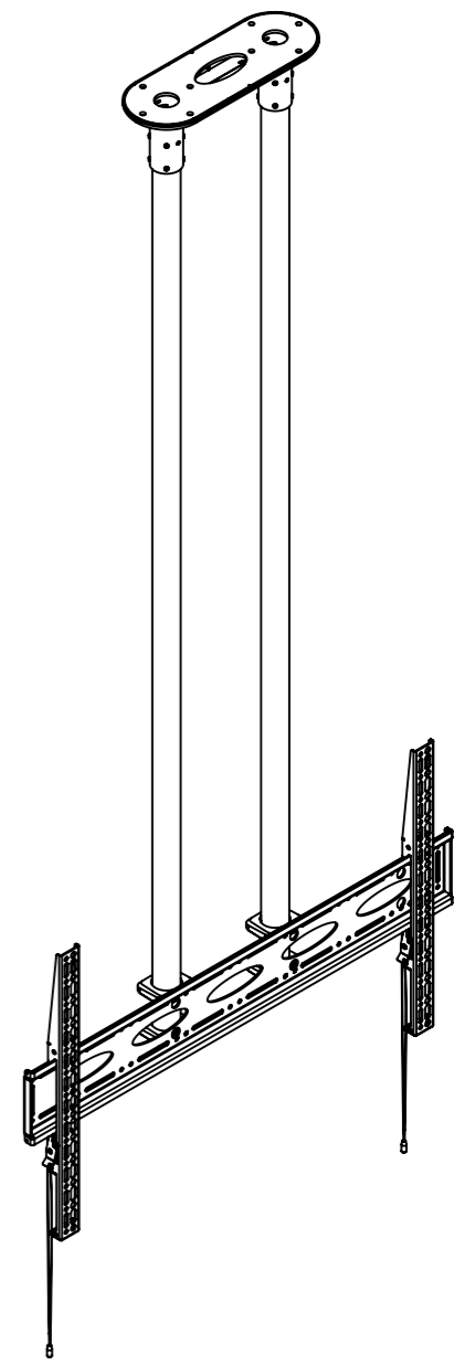
ISOMETRIC VIEW SCALE: 1 : 15
