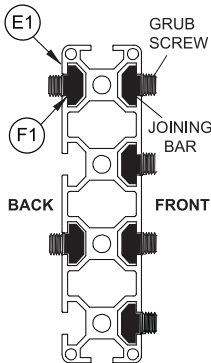
a. BT8390-WFK2 Joining Bar assembly
