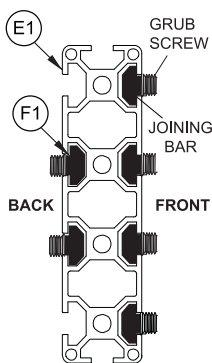
b. BT8390-CFK Joining Bar assembly
