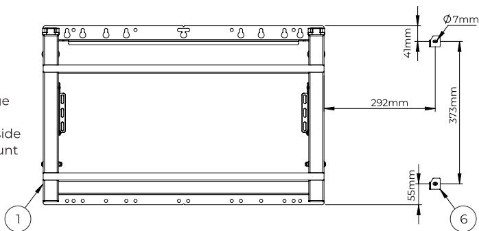
Right Sided Tray Assembly
