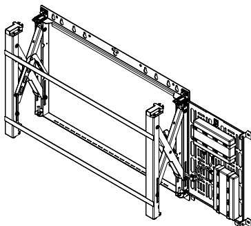
Right Sided Tray Assembly
