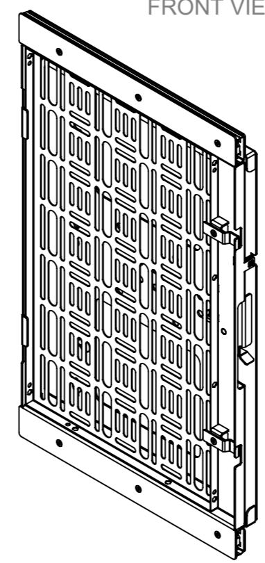
ISOMETRIC VIEW PORTRAIT CONFIGURATION - CLOSE
