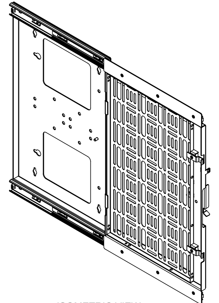
ISOMETRIC VIEW PORTRAIT CONFIGURATION - OPEN
