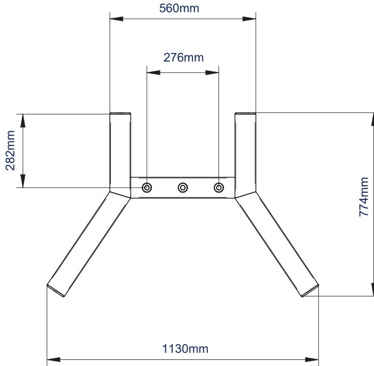
BT4003 BASE
