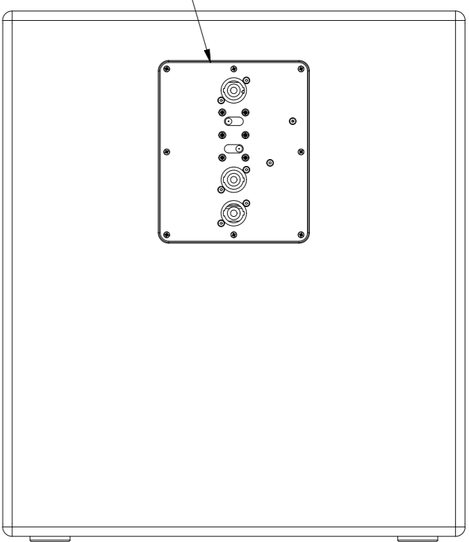
rear view
