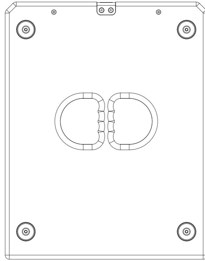
bottom view
