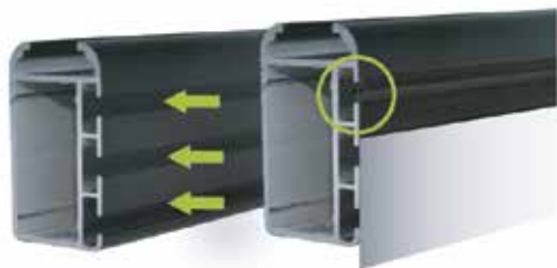
Frame assembly
